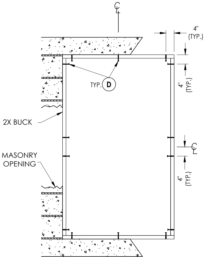
BUCK ANCHORING
